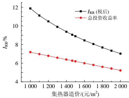
图4 内部收益率(I RR )随集热器造价的变化 Fig. 4 Changing of IRR with collector prices
