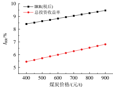
图6 内部收益率(I RR )随煤价的变化 Fig. 6 Changing of I RR with coal prices
