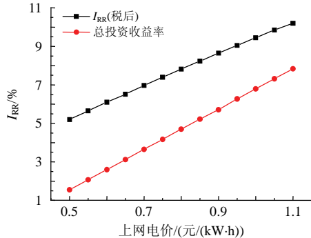
图5 内部收益率(I RR )随太阳能电价的变化 Fig. 5 Changing of IRR with electricity prices
